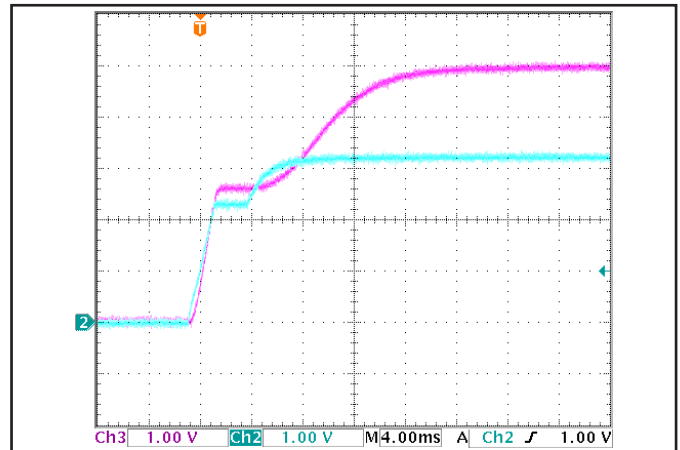
Figure 10: Management Power turn on transient at 50% load (4ms/div). Load capacitance: 10µF ceramic capacitor. Ch 2: 3.3Vout (1V/div). Ch 3: 5.0Vout (1V/div).
