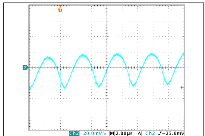
Figure 12: 3.3Vout ripple at nominal input voltage at rated load current (20mV/div). Load capacitance: 10µF ceramic capacitor. Bandwidth: 500MHz.
