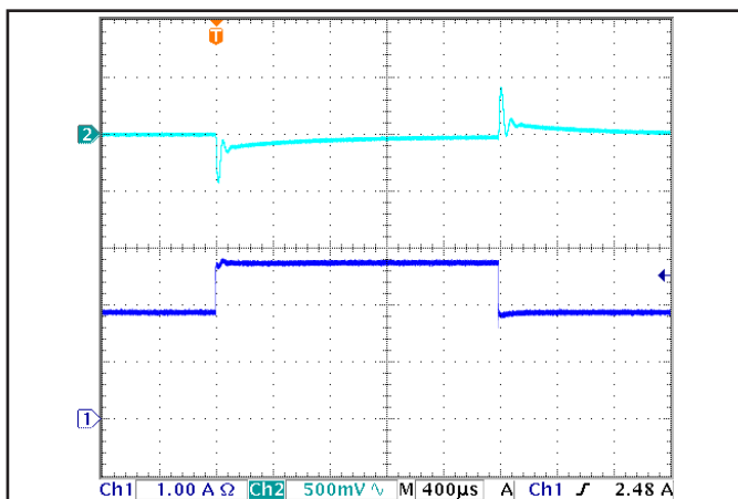
Figure 11: 3.3Vout response to a step-change in load current (50%-75%-50% of Iout(max); dI/dt = 1A/us). Load capacitance: 10µF ceramic capacitor. Top trace: 3.3Vout (500mV/div). Bottom trace: Iout (1A/div).
