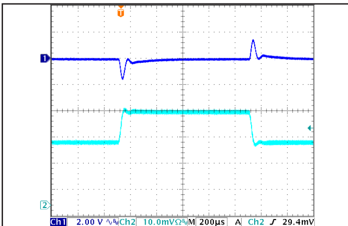
Figure 5: Output voltage response to step-change in load current (50%-75%-50% of Iout(max); dI/dt = 0.1 A/µs). Load cap: 1 µF Ceramic capacitor. Ch 1: Vout, Ch 2: Iout (2A/div).
