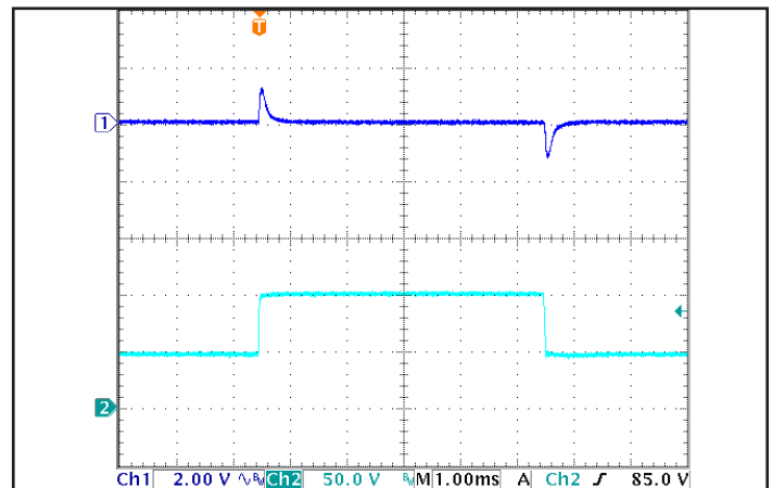
Figure 6: Output voltage response to step-change in input voltage (1000 V/ms). Load cap: 1 µF Ceramic capacitor. Ch 1: Vout, Ch 2: Vin.
