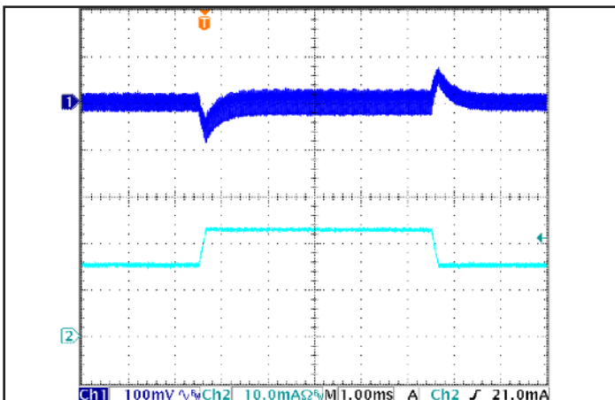
Figure 5: Output voltage response to step-change in load current (50%-75%-50% of Iout(max)); dI/dt = 0.1 \text{ A}/\mu\text{s} . Load cap: 15 \mu\text{F} tantalum and 1 \mu\text{F} ceramic capacitors. Ch 1: Vout, Ch 2: Iout (20 A/div).
