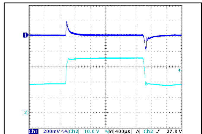
Figure 6: Output voltage response to step-change in input voltage (300 V/ms). Load cap: 100 \mu F , electrolytic output capacitance. Ch 1: V_{out} (200 mV/div), Ch 2: V_{in} (10 V/div).
