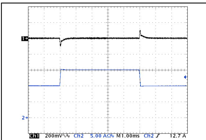
Figure 5: Output voltage response to step-change in load current (50%-75%-50% of I_{out(max)} ; dI/dt = 0.1 A/\mu s ). Load cap: 1 \mu F ceramic and 15 \mu F tantalum capacitors. Ch 1: V_{out} (200 mV/div), Ch 2: I_{out} (5 A/div).
