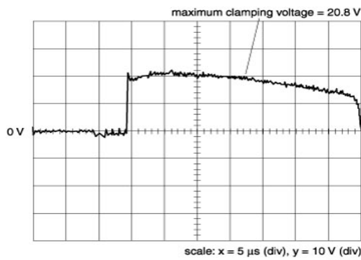
VRS0402SR55R500N Clamping Voltage Spec. 22 Typical 20.8V
