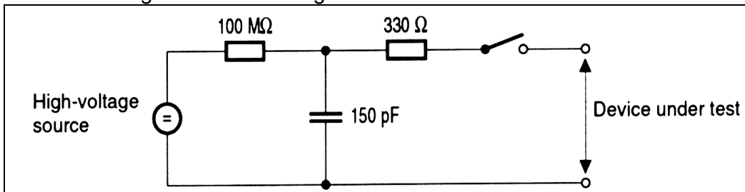
Fig3. ESD discharge circuit
