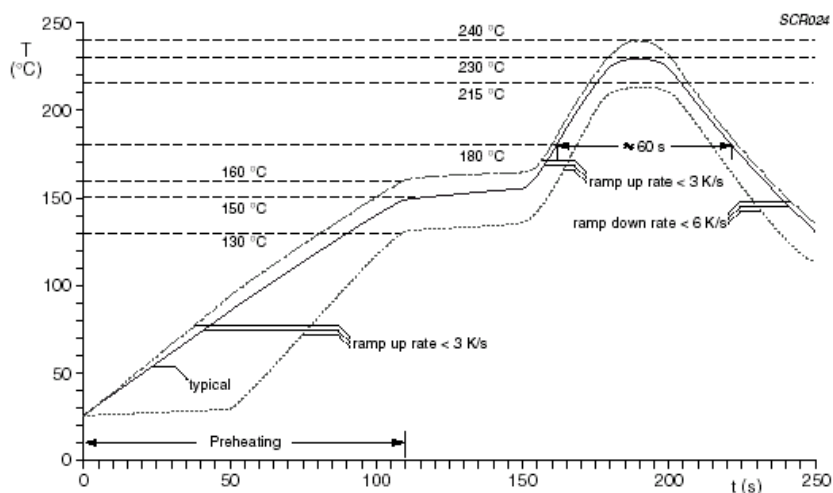
Fig. 6 Infrared soldering, forced air convection reflow soldering-temperature/time profile for SnPb solders
