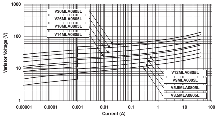
FIGURE 6. LIMIT V-I CHARACTERISTIC FOR V3.5MLA0805L TO V30MLA0805L
