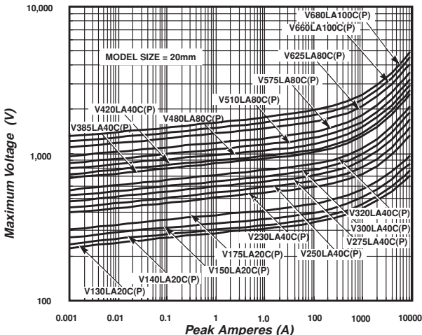
Figure 5. Maximum Clamping Voltage for 20mm Parts (V130LA20C(P) -V680LA100C(P))
