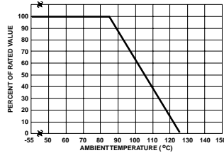
FIGURE 1. CURRENT, ENERGY AND POWER DERATING CURVE
