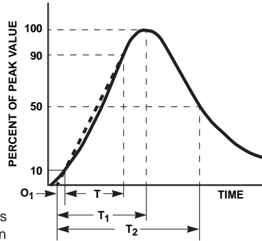
FIGURE 2. PEAK PULSE CURRENT TEST WAVEFORM
