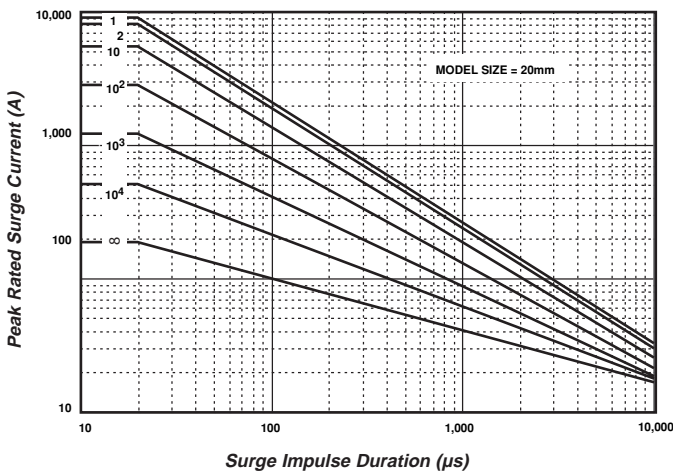
Figure 9. Repetitive Surge Capability for 20mm Parts (V130LA20C(P)-V680LA100C(P))
