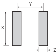
Pad Layout - Surface-mount Devices (GTCS25-XXXM-R02)
