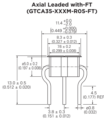
Figure G7 Three Electrode 5mm Product Dimensions
