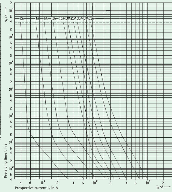
Time/current characteristics of Z-DII-Fuse-links 2 ... 63A DZ
