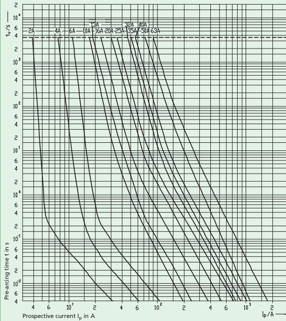
Time/current characteristics of Z-DII-Fuse-links 2 ... 63A gG(gL)
