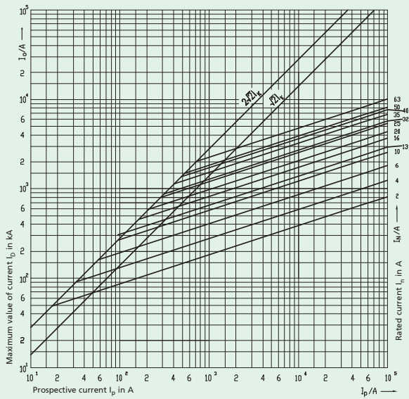
Let-through current characteristics of Z-DII-Fuse-links 2 ... 63A gG(gL)
