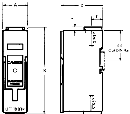
Standard Front Connected Unit
