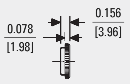
3/8 - 32 Panel Nut Bright Nickel
