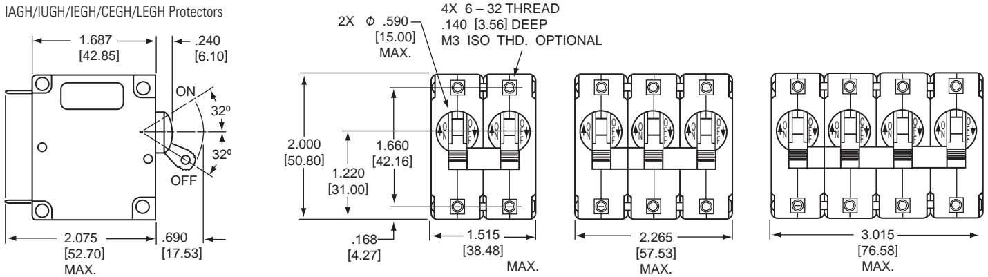
IAGH/IUGH/IEGH/CEGH/LEGH Protectors
