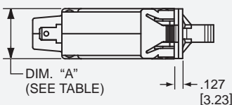
Panel Cutout Detail Panel Thickness: (See Table)
