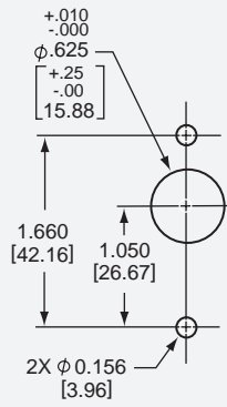
Single Pole Mounting Detail
