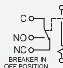
Series with Auxiliary Switch
