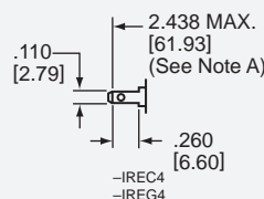
Series with Auxiliary Switch
