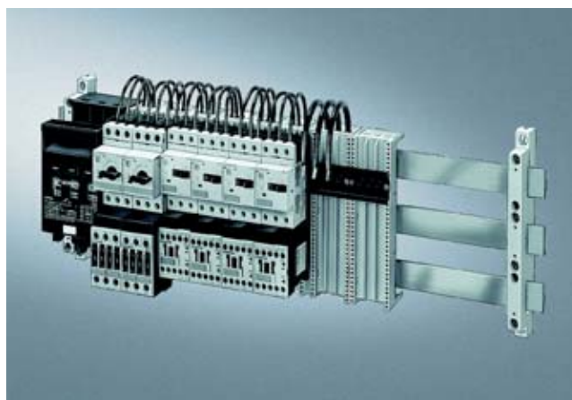
SIRIUS motor starter protectors and load feeders with busbar adapters snapped onto busbars
