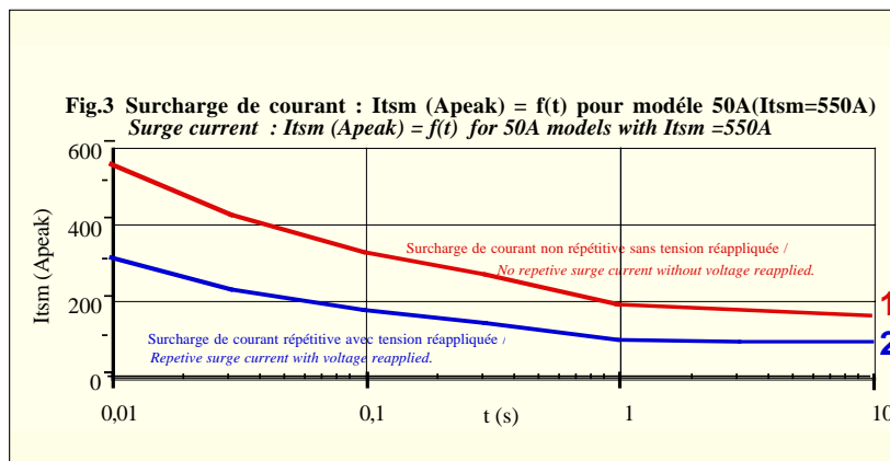
fig 3 : Courants de surcharges / Overload currents
