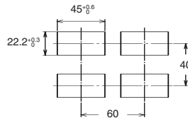
• Panel cutout
