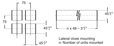
• Panel cutout
