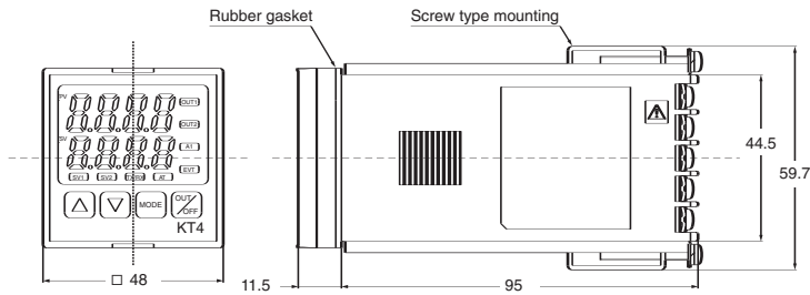
KT4 Series (unit: mm)
