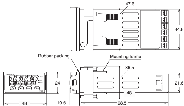
KT2 Series (unit: mm)
