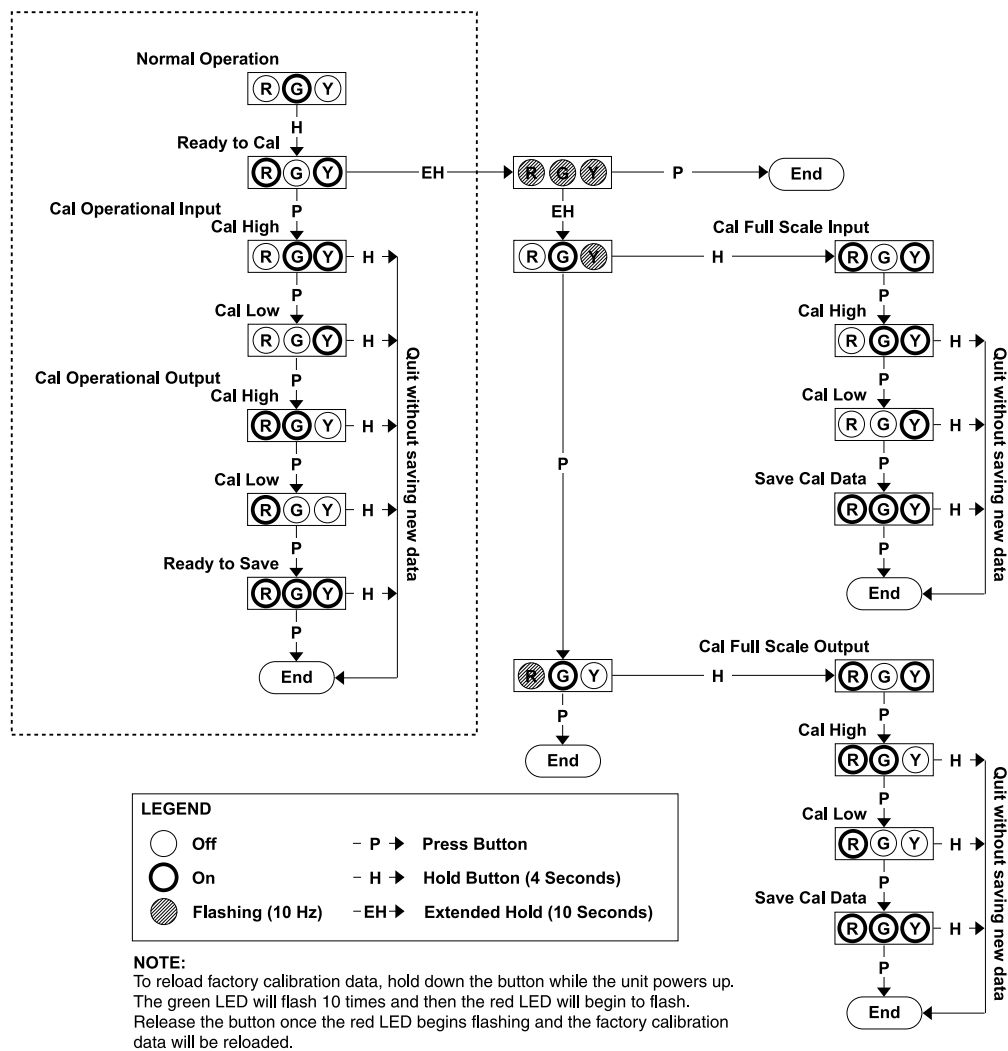
Figure 3: Switch Settings
