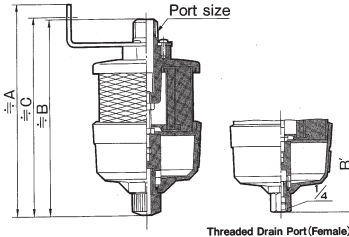
Threaded Drain Port (Female)
