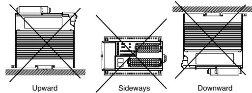
Figure 2. Incorrect Mounting Directions
