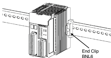
Figure 1. Correct Mounting Direction
