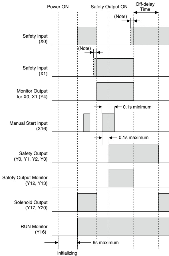
When using manual start input X16
