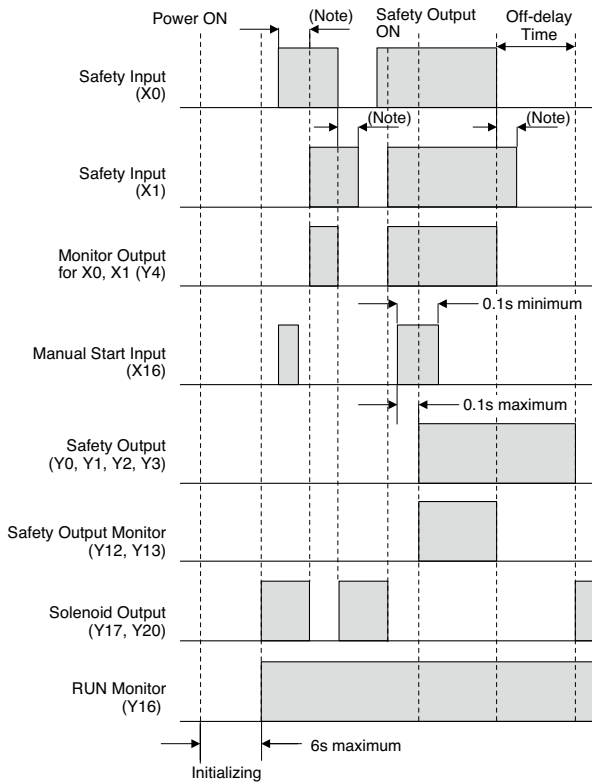
When using manual start input X16
