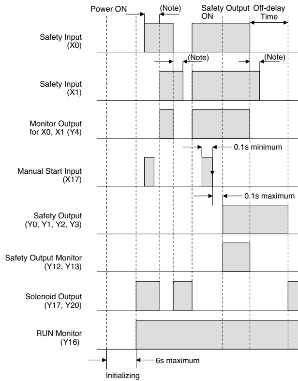
When using control start input X17
