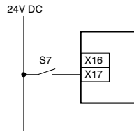
When not using some safety inputs
