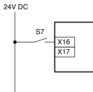
When not detecting the welding of start switch (manual start)
