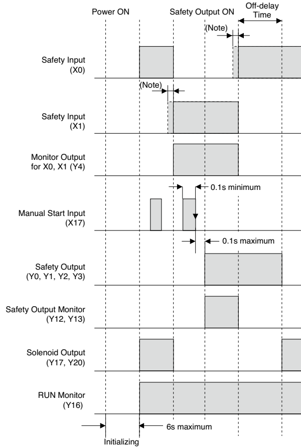
When using control start input X17
