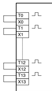
When not using some safety inputs
