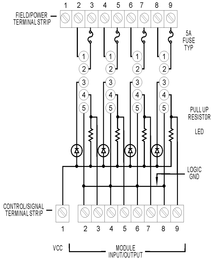
PB4 SCHEMATIC
