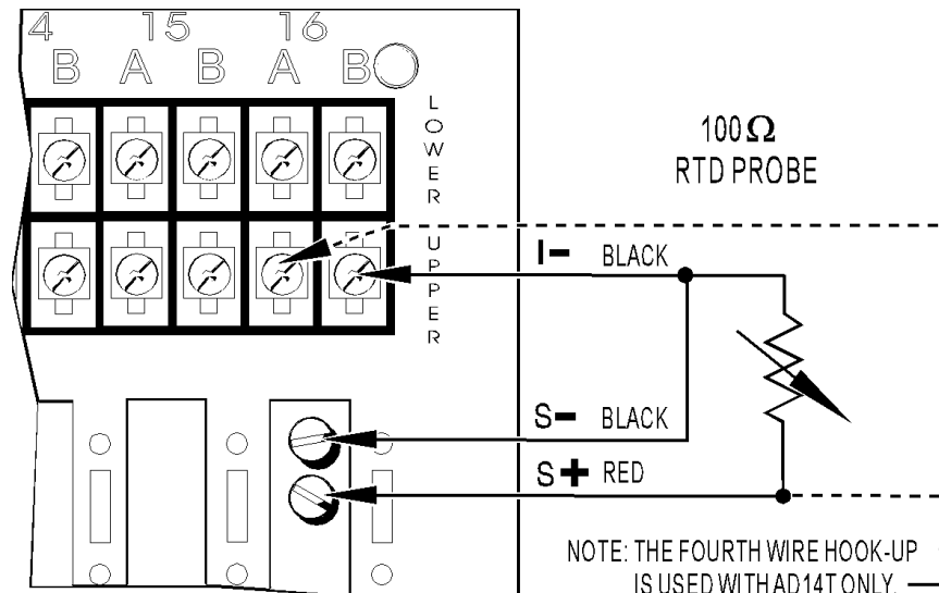
RTD CONNECTION DIAGRAM
