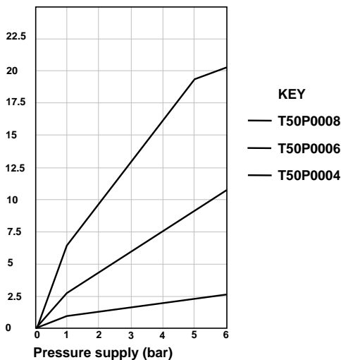
Flow measured in dm 3 /(s. bar)
