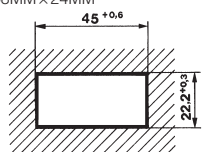
DIMENSIONS IN MM ENQUIRE FOR SEALS
