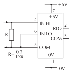
Measuring current.
