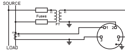
Fig. 2 Model 077-137 360° Dynamometer Power Factor Indicator Single Phase.
