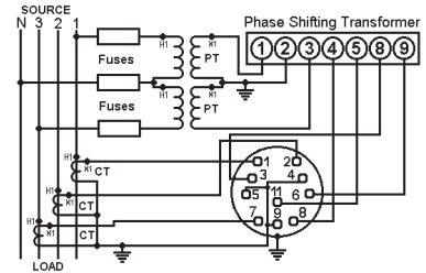
Fig. 34 Model 077-319 Varmeter 3 Phase 4 Wire Unbalanced Load.
