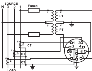
Fig. 28 Models 077-219, 077-KHG 078-219J, 078-KHGJ, 079-219 Wattmeter 3 Phase 4 Wire Unbalanced Load.
