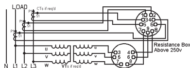
Fig. 7 Model 078-136B 360° Dynamometer Power factor Indicator 3 Phase 3 or 4 Wire Unbalanced Load.
