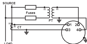
Fig. 21 Models 077-215, 077-KHB 078-215J, 078-KHBJ, 079-215 Wattmeter Single Phase.
