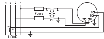
Fig. 15 Models 075-427, 077-427 078-427J, 079-427 Electronic Phase Angle Meter 3 phase 3 or 4 wire Balanced Load.
