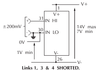
Split supply operation.
