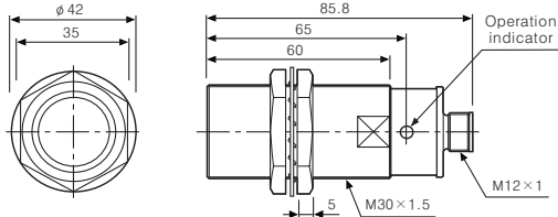
●PRCML30-10D□ / PRCML30-10A□
