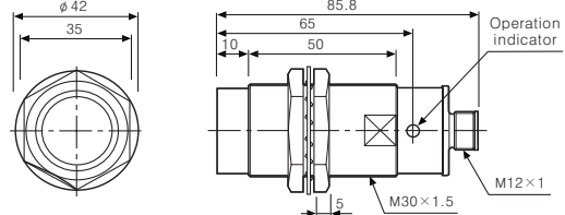
●PRCML30-15D□ / PRCML30-15A□
