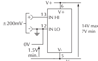
Check Links 1, 3 & 4 are SHORTED. Split supply operation (DPM 160).
