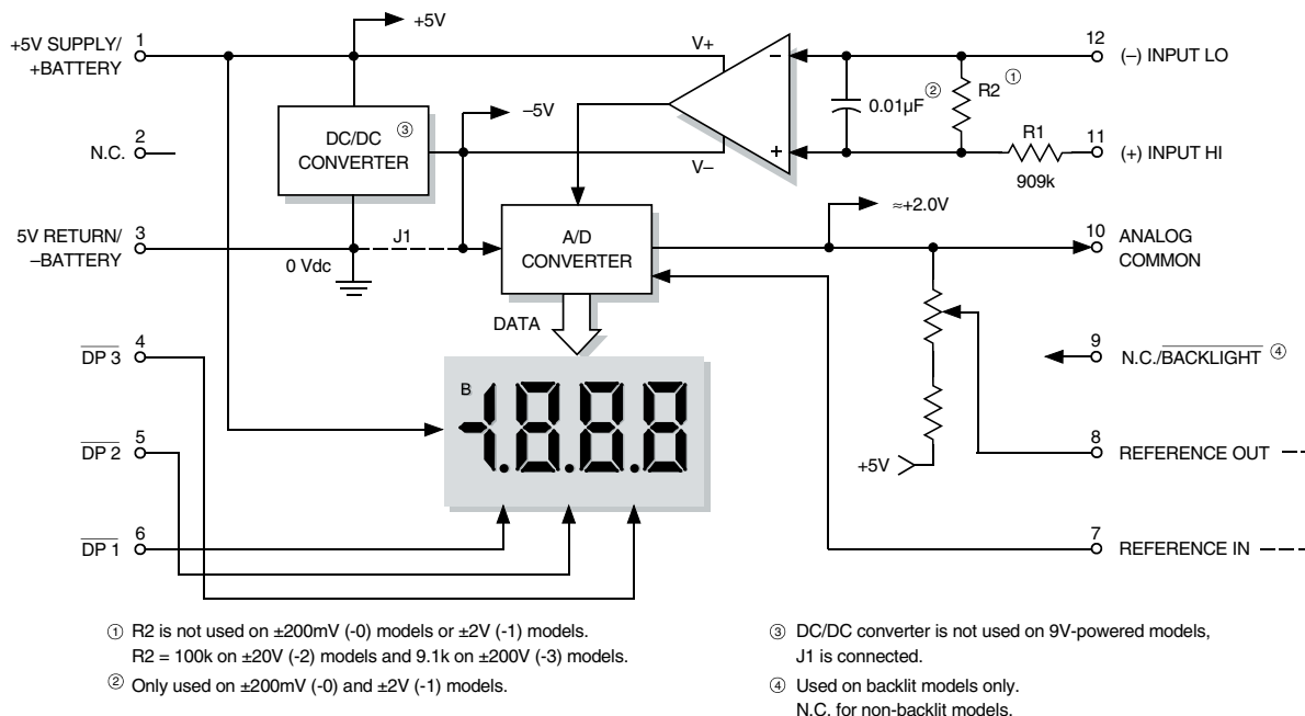
Figure 1. DMS-20LCD Series Simplified Schematic
