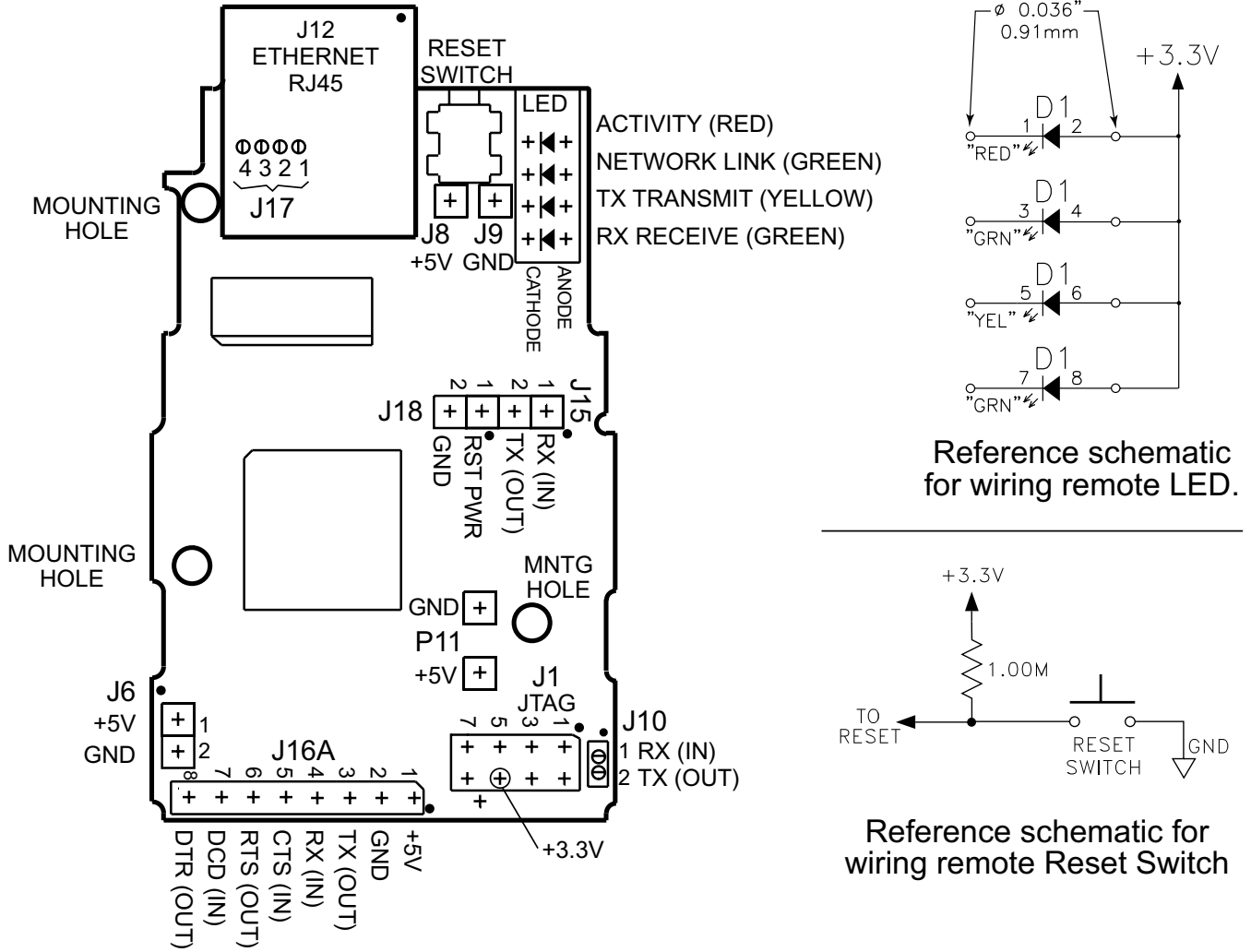
Figure 2.3 Parts of the iServer Unit
