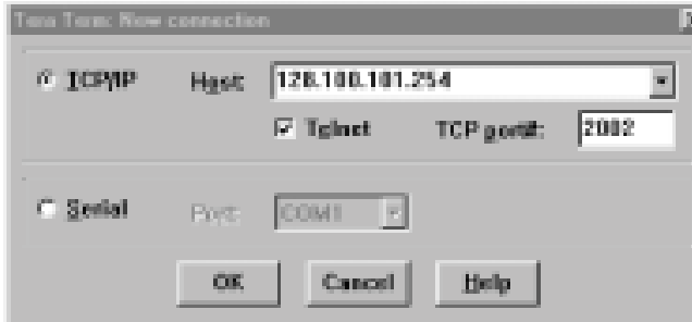
Figure 4.19 Tera Term Telnet Connection Screen
