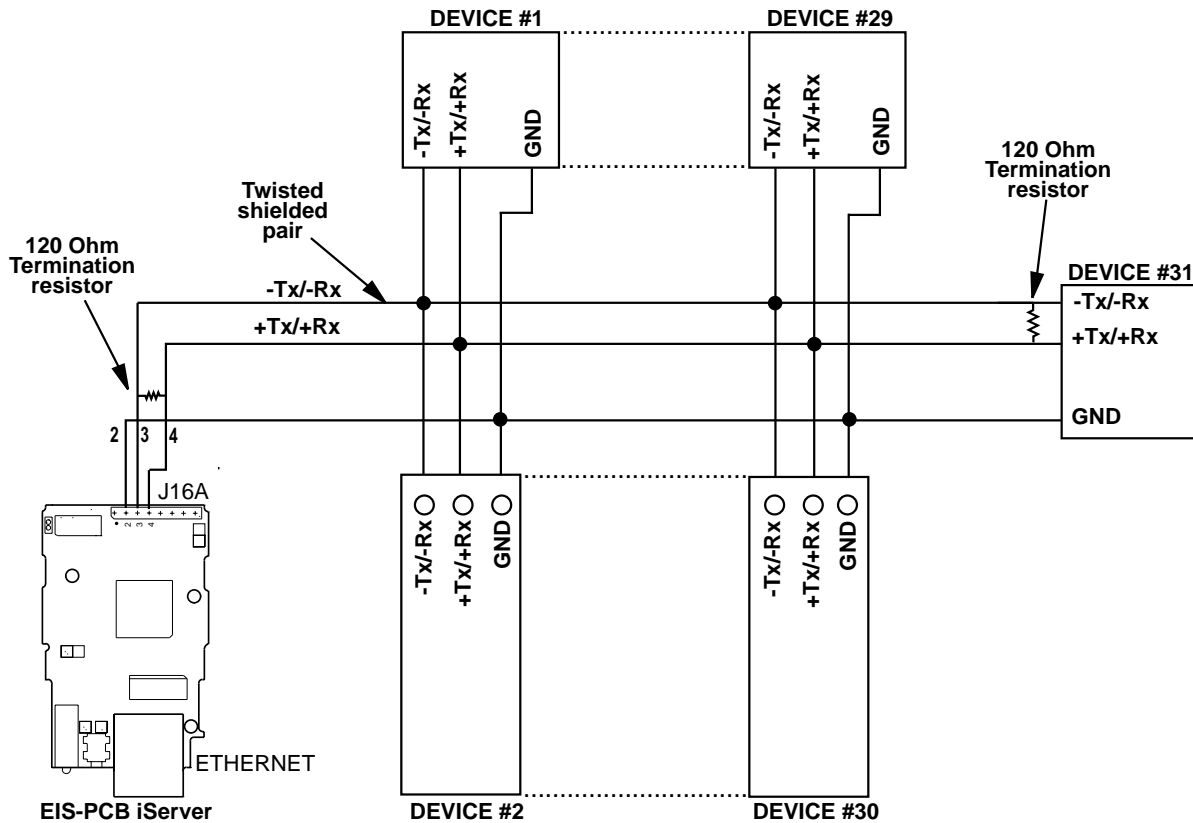
Figure 2.5 Multi-point, Half-Duplex RS485 Wiring
