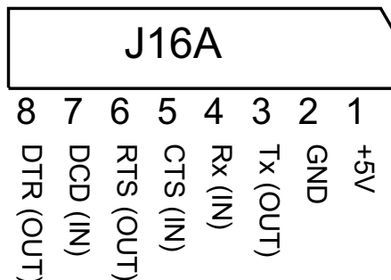
Figure 2.4 J16A Connector
