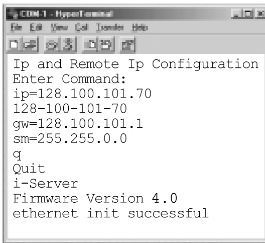
Figure 4.14 Setting the IP address via the Serial Port
