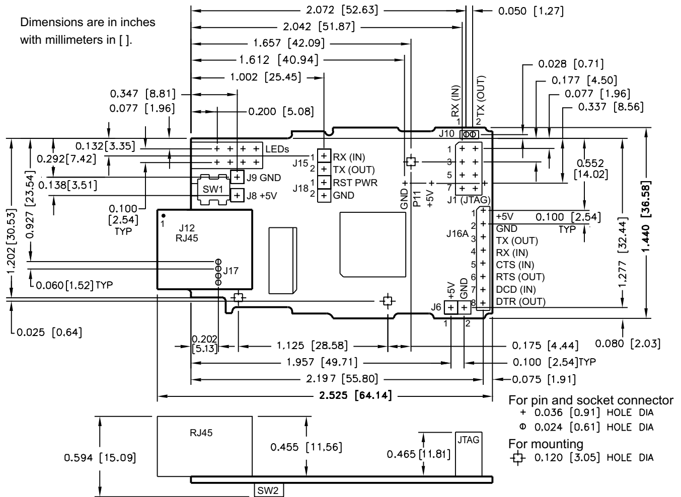
Figure 2.1 Mounting
