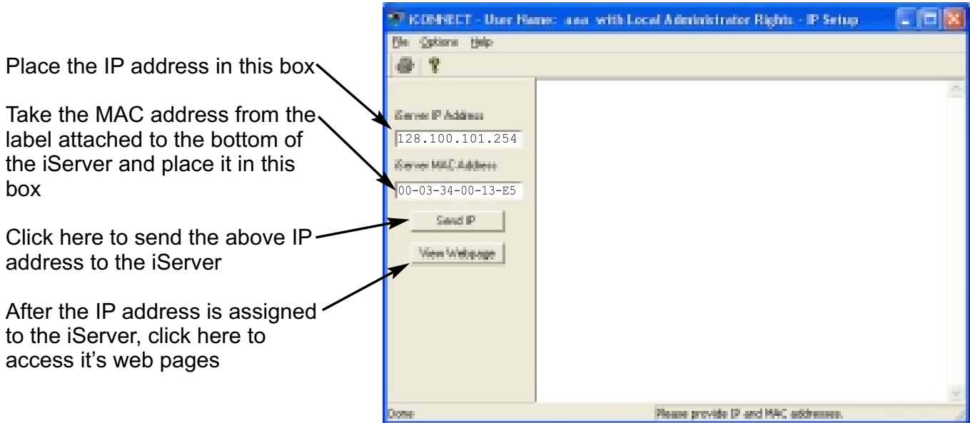
Figure 4.2 Assigning an IP Address using iCONNECT
