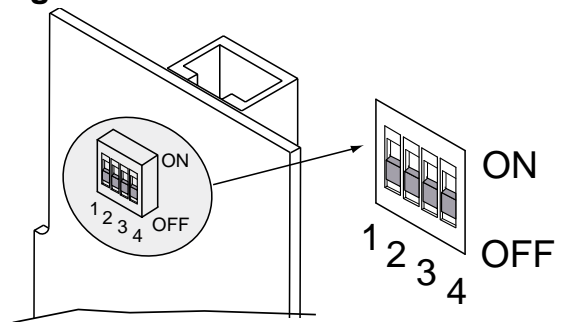
Figure 2.2 DIP Switches
