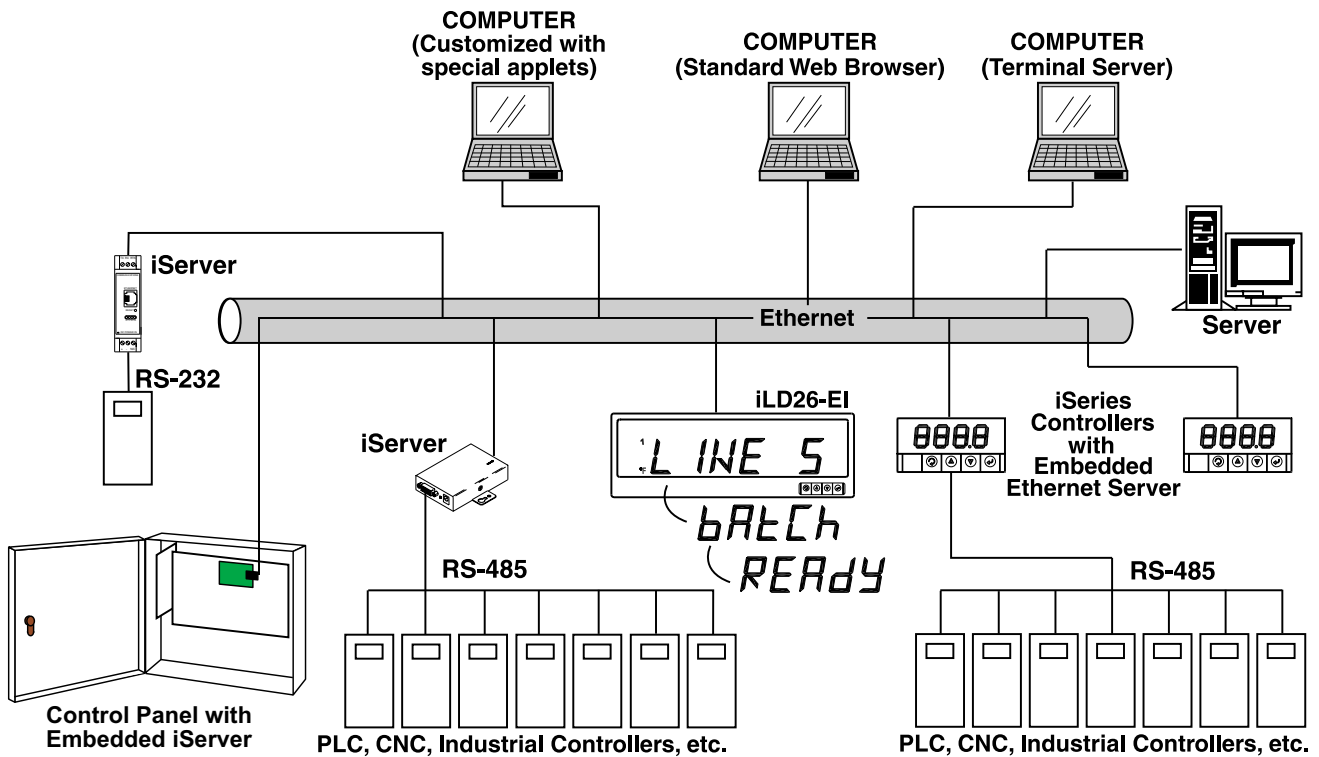
Figure 1.1 Accessing devices over the Ethernet
