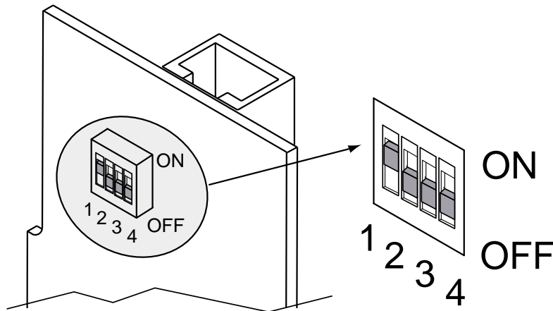
Figure 4.13 DIP switch #1 switch #1 shown in "ON" position
