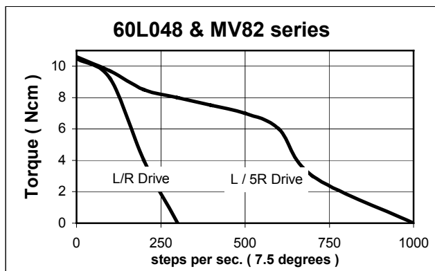
Uni-polar drive
