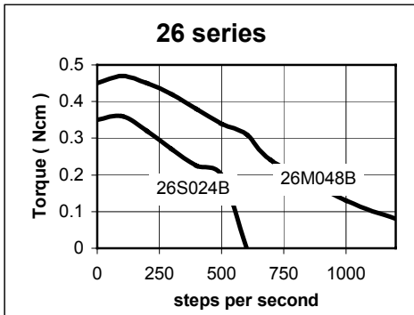
Uni-polar drive
