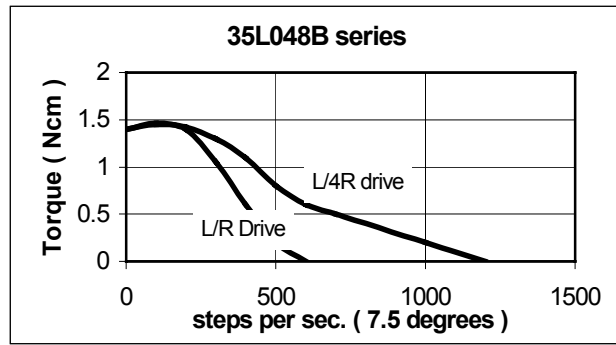
Uni-polar drive
