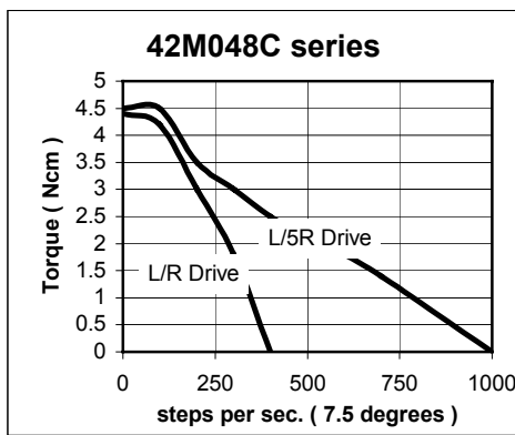
Uni-polar drive
