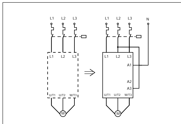
Fig. 2 For voltages higher than 480 VAC
