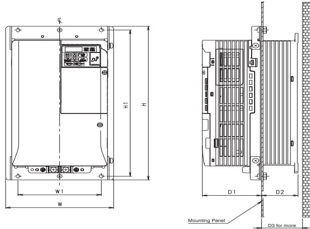
Heatsink External Mounting Attachment
