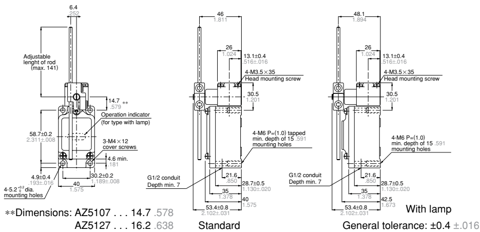
AZ5107 AZ5127 (O.T. amplified) Weight: 252g
