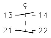
Switching symbol
