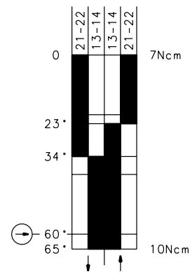
Switching diagram
