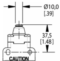
Figure 2. Pin plunger
