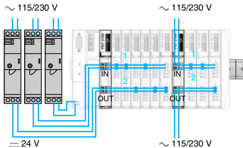
Configuration with standard PDM
