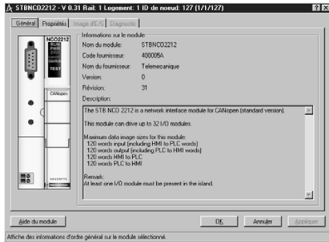
CANopen bus interface NIM module
