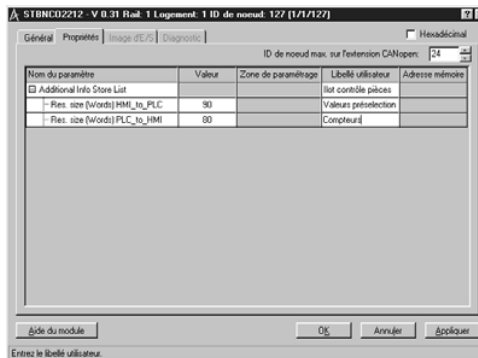
STB NCO 2212 CANopen bus interface module
