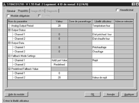
STB ACO1210 module with 2 analog output channels
