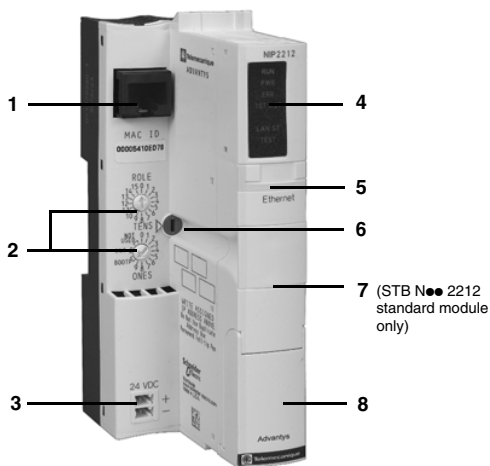
Interface modules with network/bus address selectors.
