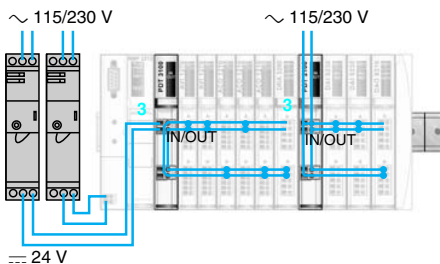
Configuration with basic PDM
