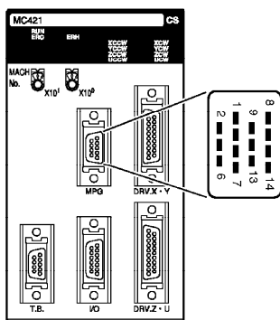
CS1W-MC421
