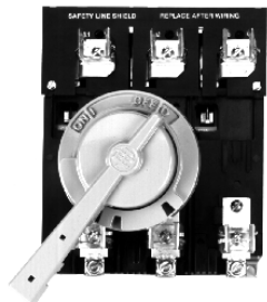
NEMA-Style Rotary Handle Disconnect Switch
