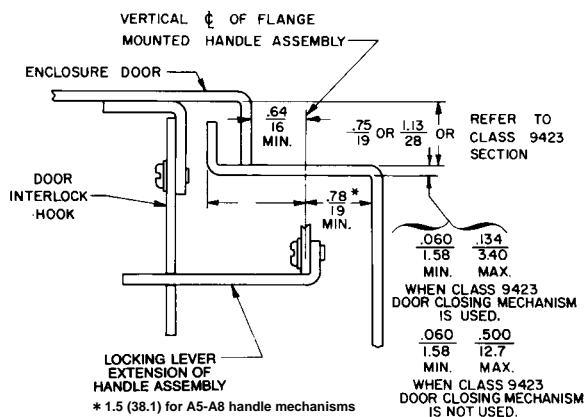
Flange Details
