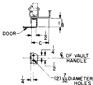
Bolted Construction
