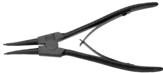
3711 Outside Circlip pliers straight
