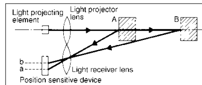
Fig. 1 Optical triangulation range measurement method
