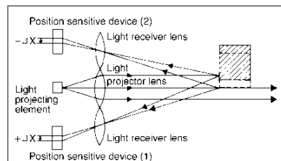
Fig. 2 Triple beam range measurement method
