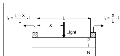
Fig. 4 PSD (position sensitive device) construction
