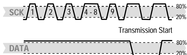
Figure 13: Connection Reset Sequence
