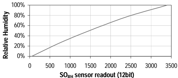
Figure 18: Conversion from SO RH to relative humidity
