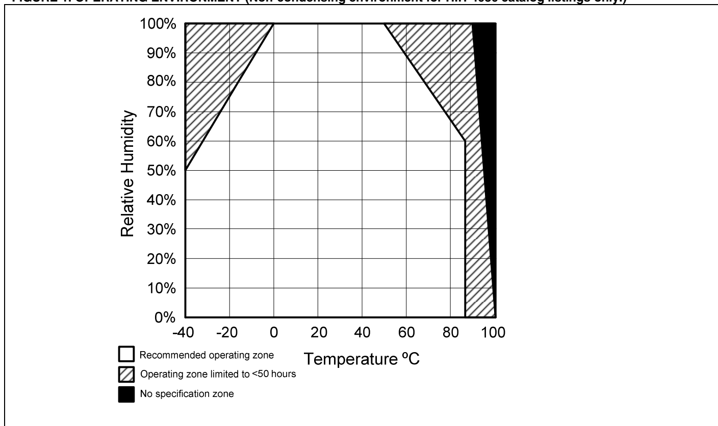
FIGURE 1. OPERATING ENVIRONMENT (Non-condensing environment for HIH-4030 catalog listings only.)
