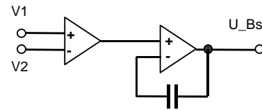
Principle of the heating controller
