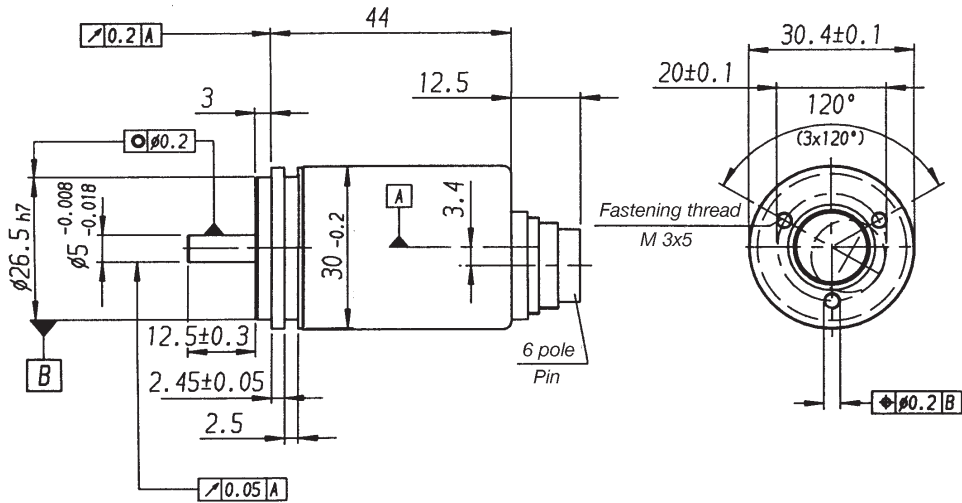
Synchro flange, BINDER
