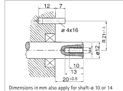
Mounting E (Blind shaft)
