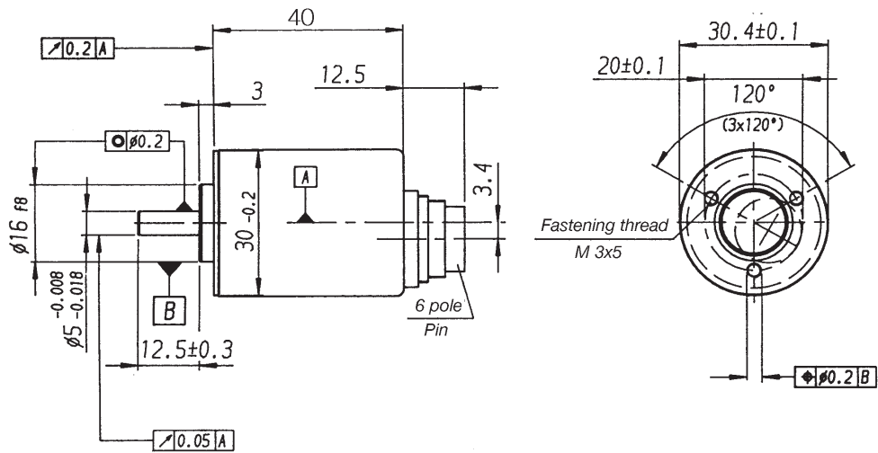
Round flange, BINDER
