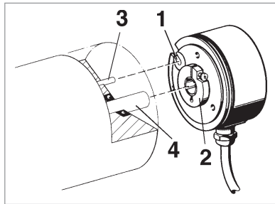
Mounting of version F, D (Clamping shaft)
