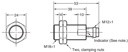
E2A-M18KS05-M1-□□/E2A-S18KS05-M1-□
