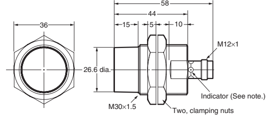
E2A-M30KN18-M1-□□/E2A-S30KN18-M1-□
