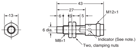
E2A-S08KN02-M1-□□
