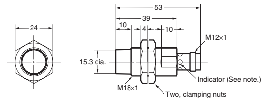
E2A-M18KN10-M1-□□/E2A-S18KN10-M1-□
