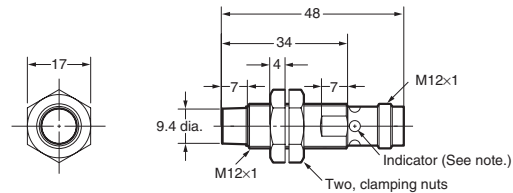
E2A-M12KN05-M1-□□/E2A-S12KN05-M1-□
