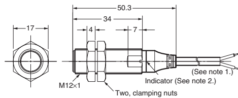
E2A-M12KS02-WP-□□/E2A-S12KS02-WP-□
