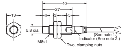
E2A-S08KN02-WP-□□
