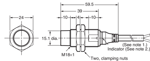
E2A-M18KN10-WP-□□/E2A-S18KN10-WP-□
