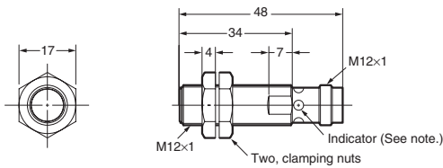
E2A-M12KS02-M1-□□/E2A-S12KS02-M1-□
