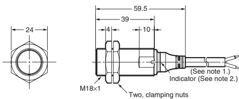
E2A-M18KS05-WP-□□/E2A-S18KS05-WP-□
