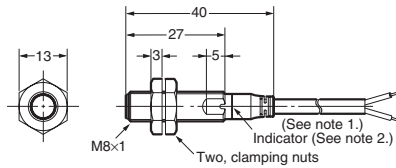
E2A-S08KS01-WP-□□
