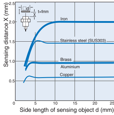
E2A-M12□N05/E2A-S12□N05
