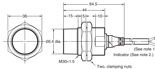
E2A-M30KN18-WP-□□/E2A-S30KN18-WP-□
