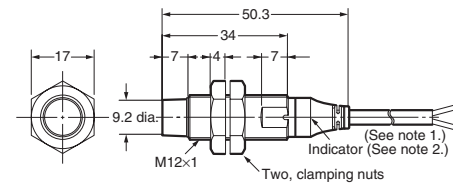
E2A-M12KN05-WP-□□/E2A-S12KN05-WP-□
