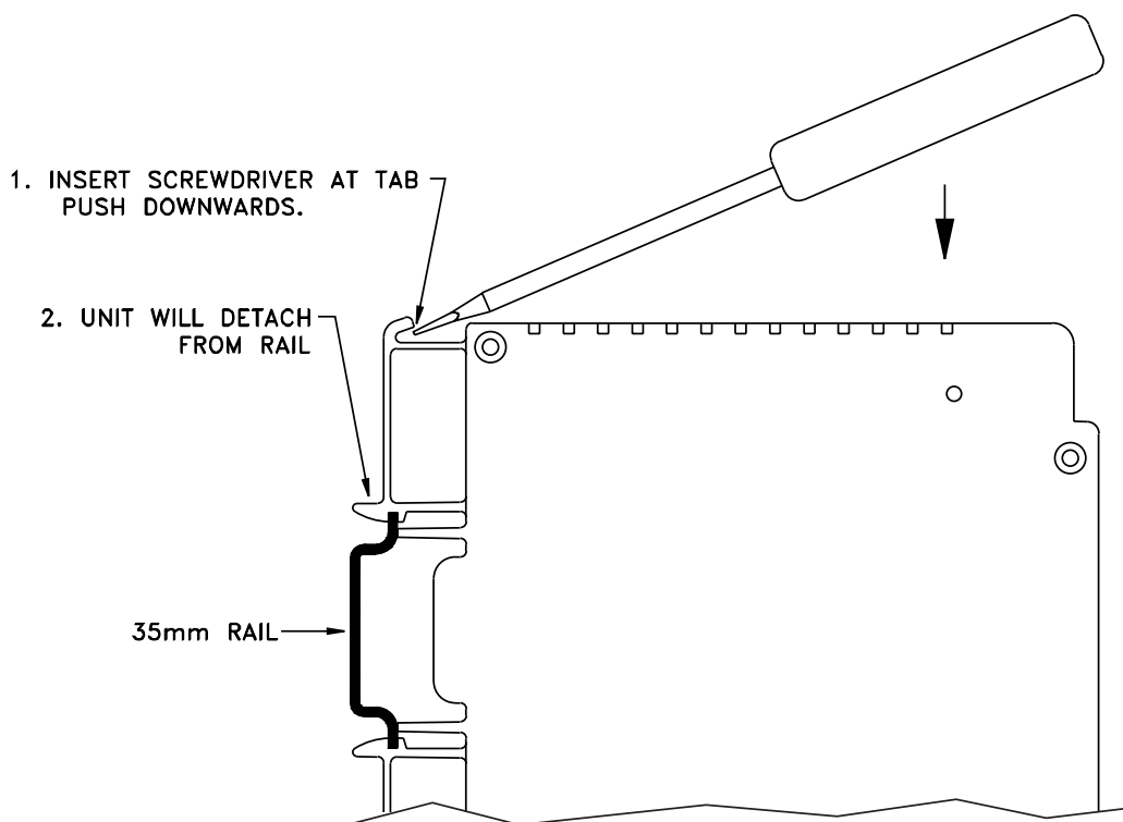
Figure 2.3 Removal - DIN Rail iServer
