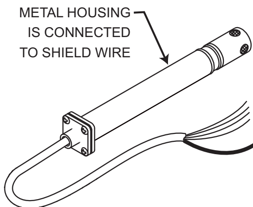
Figure 2.8 Industrial Probe Wiring Hookup
