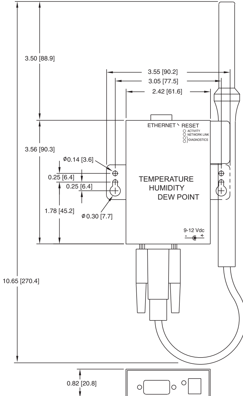
Figure 2.1 Mounting - Wall Mount iServer
