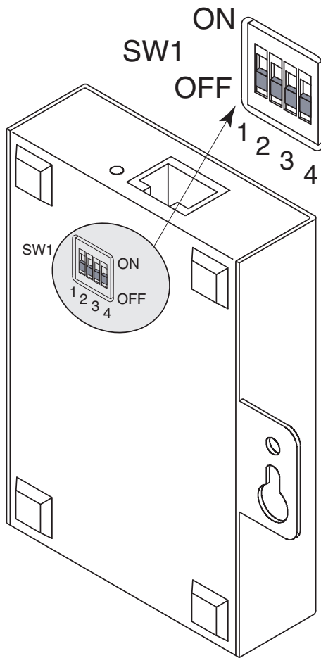
Figure 2.4a DIP Switch Wall Mount iServer
