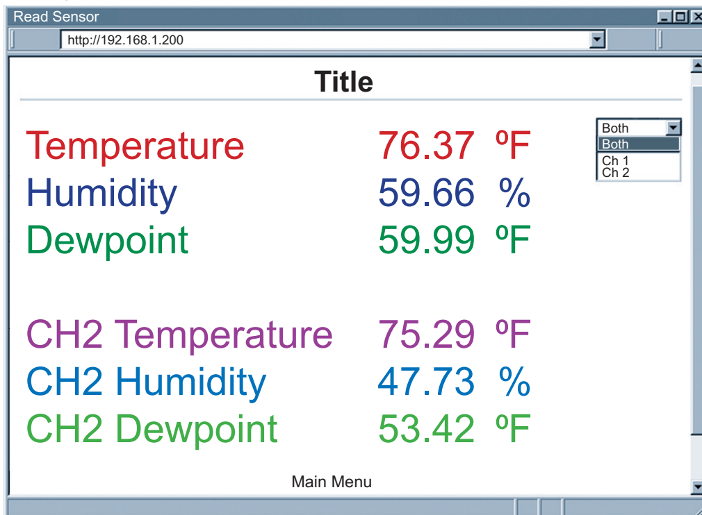
Figure 4.7 Read Sensor
