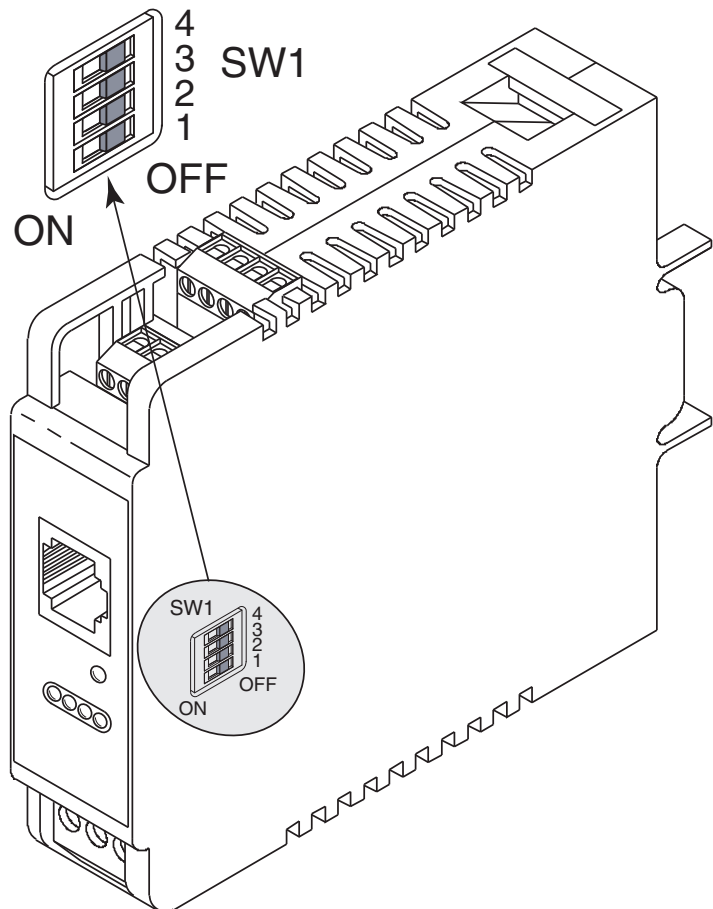
Figure 2.4b DIP Switch DIN Rail iServer
