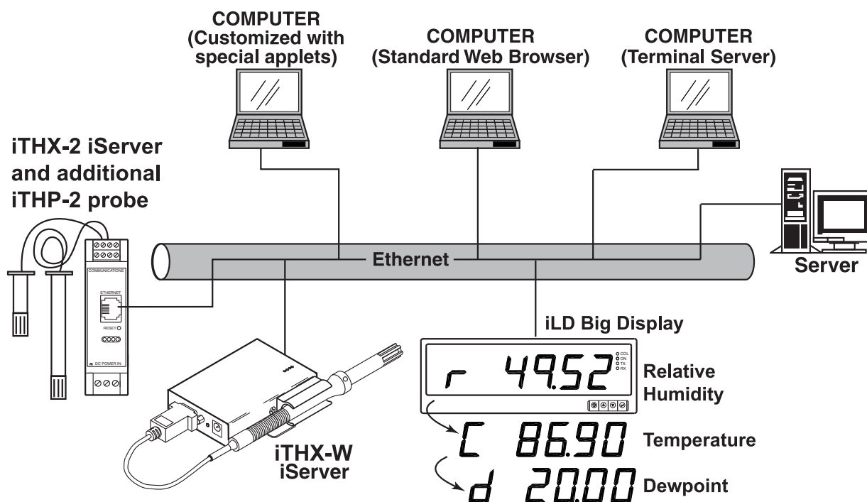
Figure 1.1 iServer with Probe on the Ethernet Network
