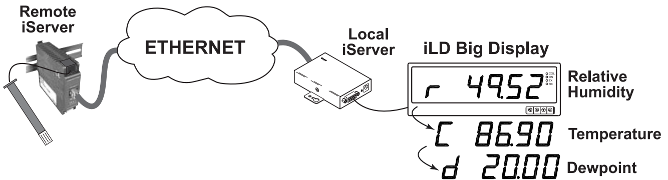
Figure 4.15 Device-to-Device Communication
