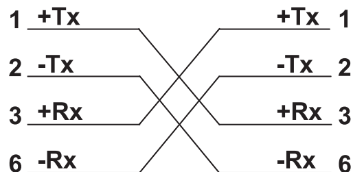
Figure 2.7 10Base-T Crossover Cable Wiring
