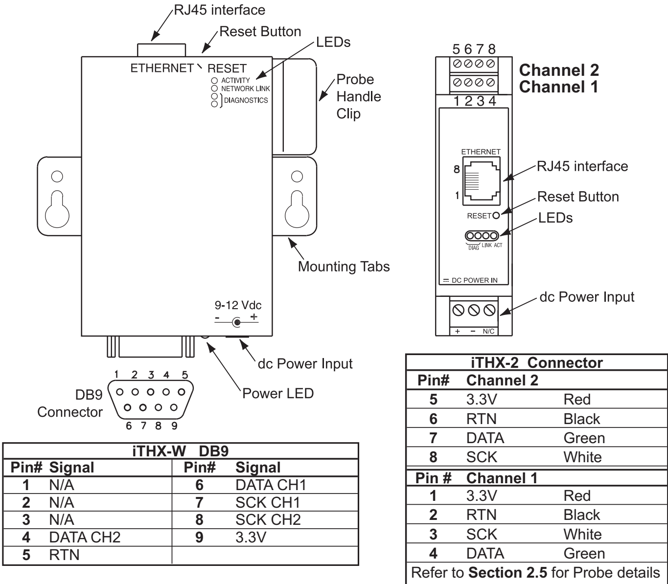
Figure 2.5 Parts of the iServer Unit
