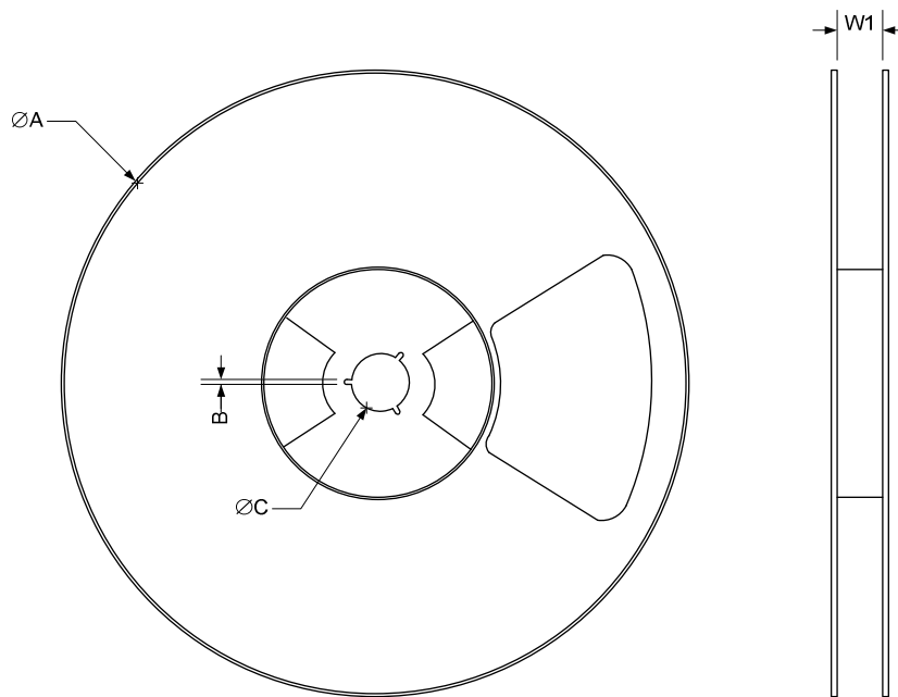
Figure 4: Reel information (drawing not to scale)
