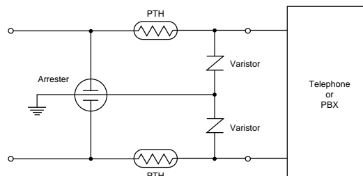
(5) Telecommunication Circuit
