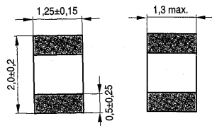
Termination TNT0397-7-E Dimensions in mm Approx. weight 13 mg
