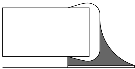
Good solder joint
